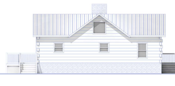
Rear Elevation
