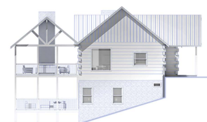
Left Elevation
